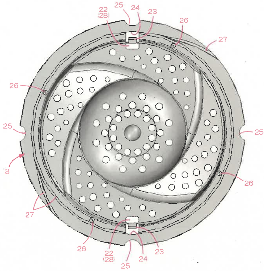
[底面图]
